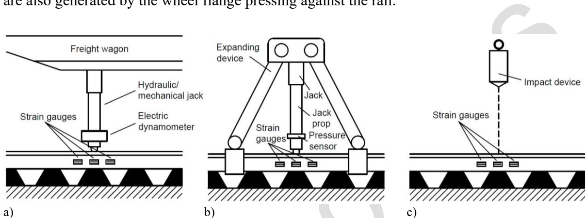
Fig. 1. Calibration systems: (a) static calibration device applied with a freight wagon, (b) static expanding calibration device, (c) dynamic impact calibration device.
