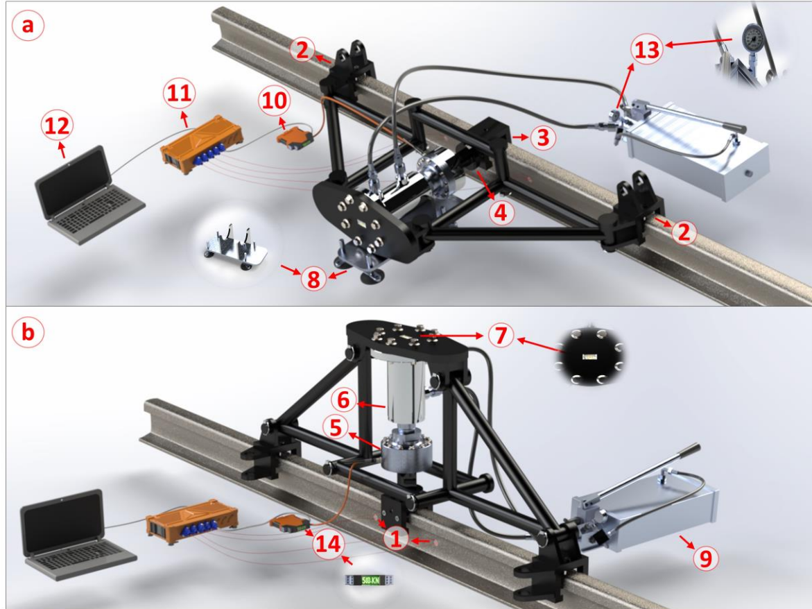
Fig. 8. Horizontal (a) and vertical (b) usage of Variant 3: 1 - strain gauges, 2 - grippers, 3 - pressure head, 4 - force apparatus, 5 - load cell, 6 - hydraulic cylinder, 7 - spirit level, 8 - horizontal support platform, 9 - hand pump, 10 - load cell transmitter, 11 - DAQ, 12 - laptop, 13 - analog gauge, 14 - digital display.
