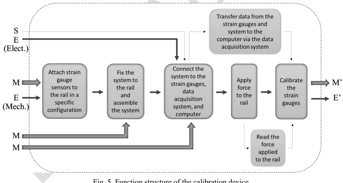
Fig. 5. Function structure of the calibration device.
