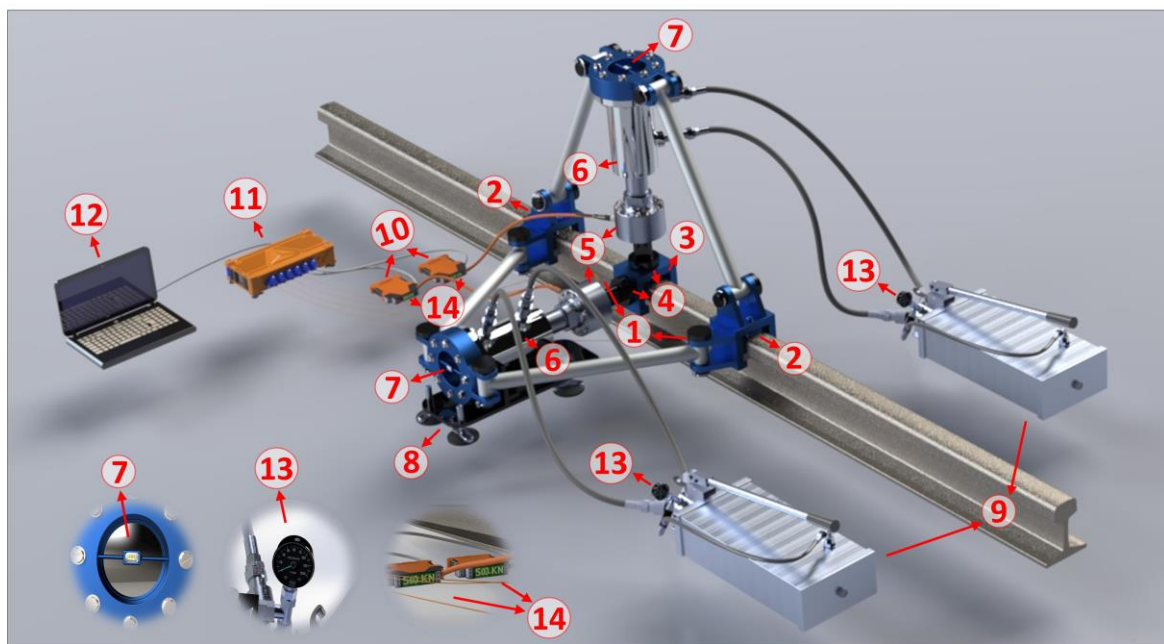
Figure 7. Variant 2: 1 - strain gauges, 2 - grippers, 3 - pressure head, 4 - force apparatus, 5 - load cell, 6 - hydraulic cylinder, 7 - spirit level, 8 - horizontal support platform, 9 - hand pump, 10 - load cell transmitter, 11 - DAQ, 12 - laptop, 13 - analog gauge, 14 - digital display.
