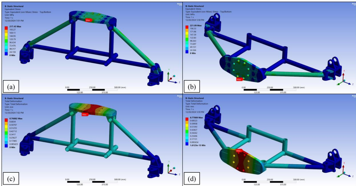
Fig. 10. Stress (a), (b) and deformation (c), (d) results for the vertical and horizontal cases.
