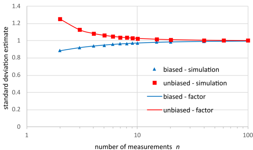
Fig. 1. The simulation results of s_{BA} and s_{UA} are shown (relatively to the unbiased s ) by symbols for a given number of measurements n and the common unbiased mean value \bar{x} . They are compared with analytical factors f_B and f_U , respectively. The simulation and analytical estimates agree to within 0.3 %.
