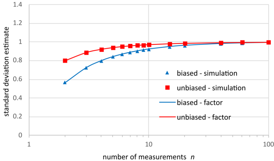
Fig. 2. The simulation results of s_{BXA} and s_{UXA} are shown (relatively to the unbiased s ) by symbols for a given number of measurements n and the evaluated biased mean values. They are compared with analytical factors f_{BX} and f_{UX} , respectively. The simulation and analytical estimates agree to within 0.3 %.
