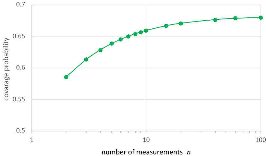
Fig. 3. The simulation results (symbols) of the average of coverage probability for the mean value biased estimates with the correct standard deviation s . The (16) is shown (as a line) for a comparison that agree to be relatively within 0.1 %. The coverage probability of about 68.27 % corresponds to the infinity number of measurements with the normal distribution.
