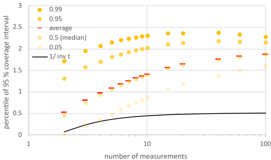
Fig. 5. The confidence interval for the coverage probability of 95 % with the scale given by the unbiased standard deviation s . Symbols represent percentiles 0.05, 0.5, 0.95, 0.99 and average of these evaluated intervals for a given number of measurements n . The reciprocal values of the inverse Student's t distribution for probability 0.05 are shown for a comparison (line).
