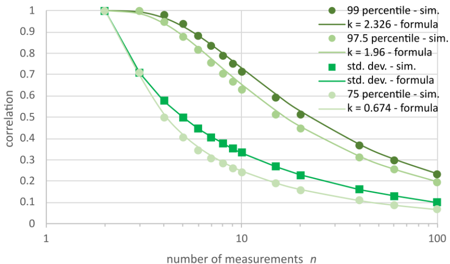
Fig. 7. The standard deviation and percentiles of simulated correlation between pairs of n uncorrelated measurements (symbols). The (21) and (23) are shown for a comparison (lines).
