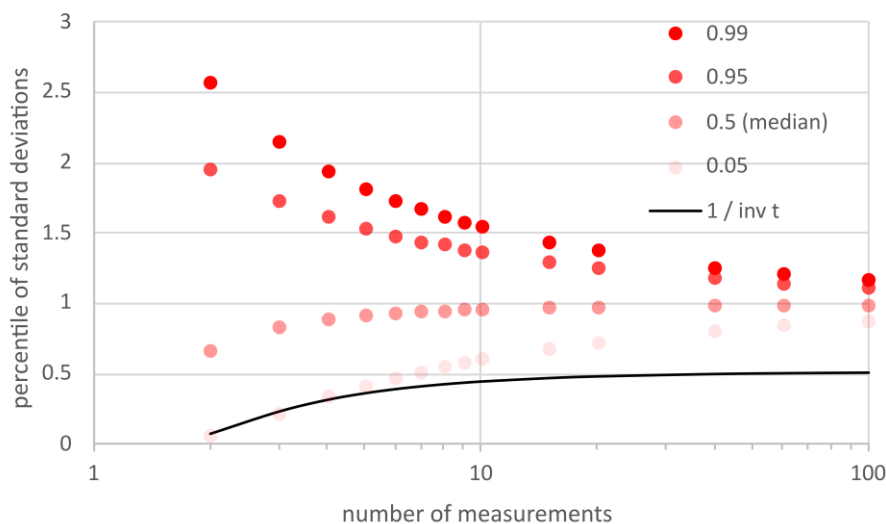
Fig. 4. The uncorrected simulation results (symbols) for percentiles of the “unbiased” standard deviations given by (10). The median is approximately (within 20 %) equal to the mean from Fig. 2. The reciprocal values of the inverse Student's t distribution for probability of 0.05 are shown for a comparison (line).
