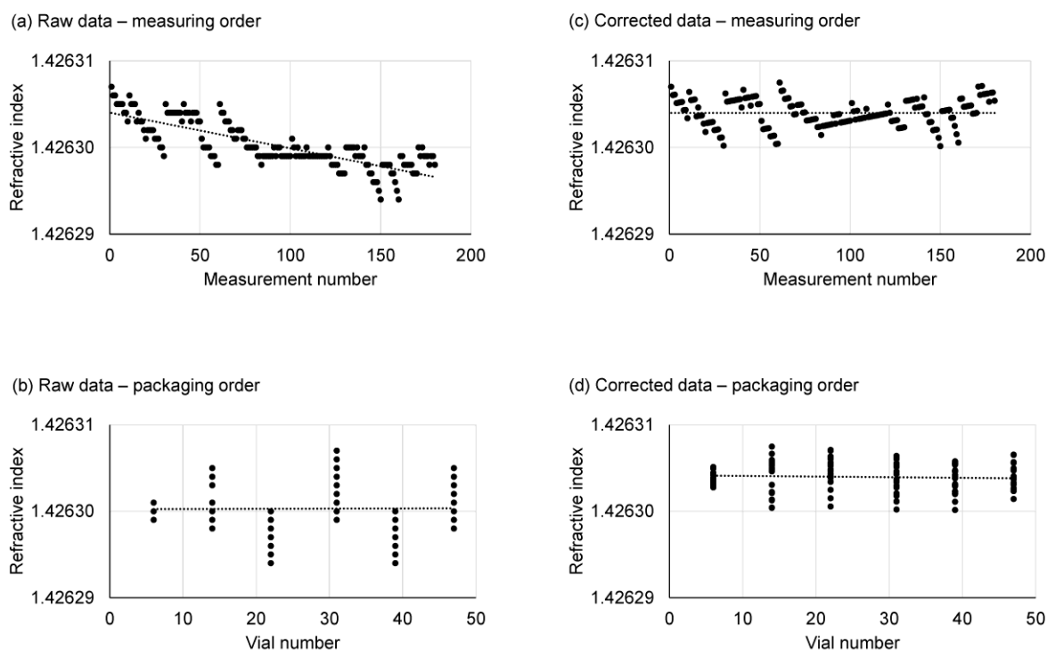
Fig. 2. Trend analysis of a batch of cyclohexane as a CRM candidate for refractive index.
