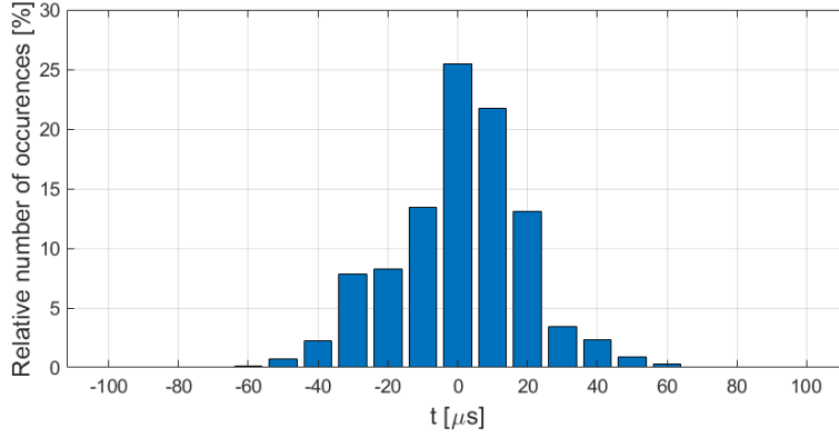
Fig. 8. Histogram of deviation of e-Czas Radio signal time of arrival measurements with respect to mean value.
