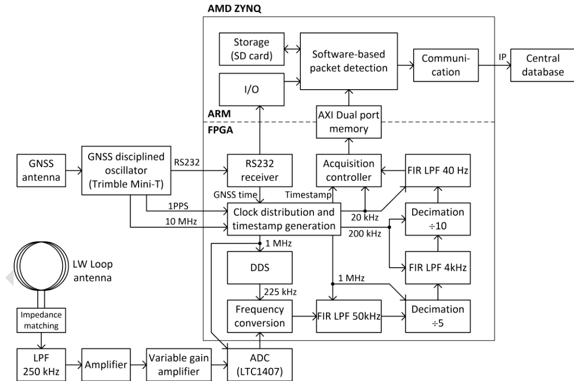
Fig. 3. Block diagram of e-Czas Radio signal receivers.
