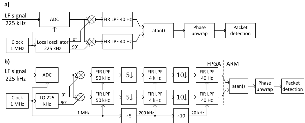
Fig. 4. General concept (a) and real implementation (b) of digital signal processing in LF receiver.
