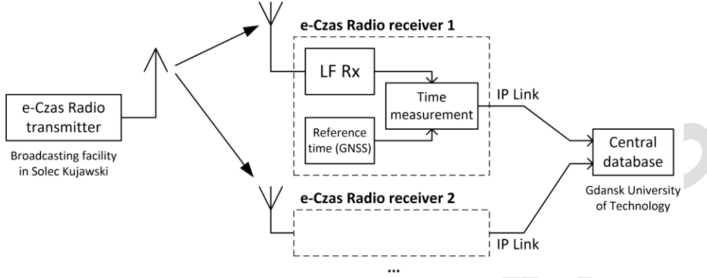
Fig. 1. Block diagram of receiver network for e-Czas Radio time dissemination performance assessment.
