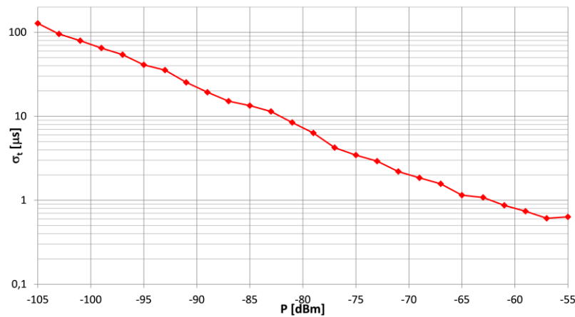
Fig. 7. Standard deviation of e-Czas packet time measurements as a function of signal power level for test signal generated using R&S SMU200.
