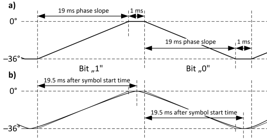
Fig. 5. Carrier phase theoretical shape a) and model used for detection of message time b).
