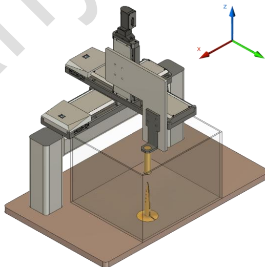
Fig. 4. 3D design of the experimental measurement setup
