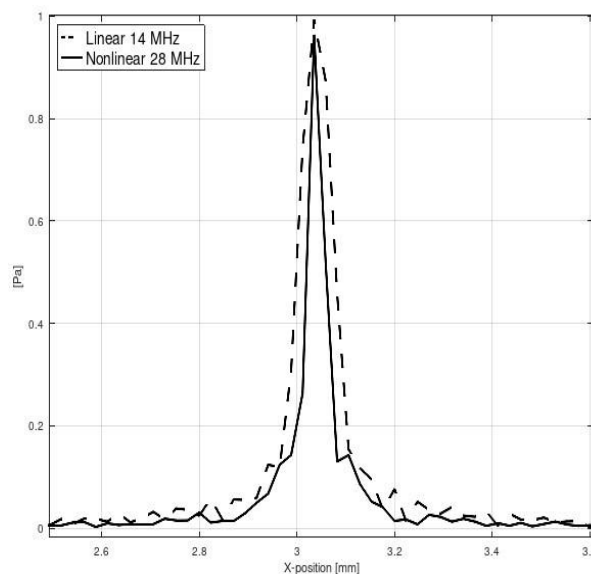
Fig. 9. Linear (14 MHz) and nonlinear (28 MHz) lateral pressure (Normalized).
