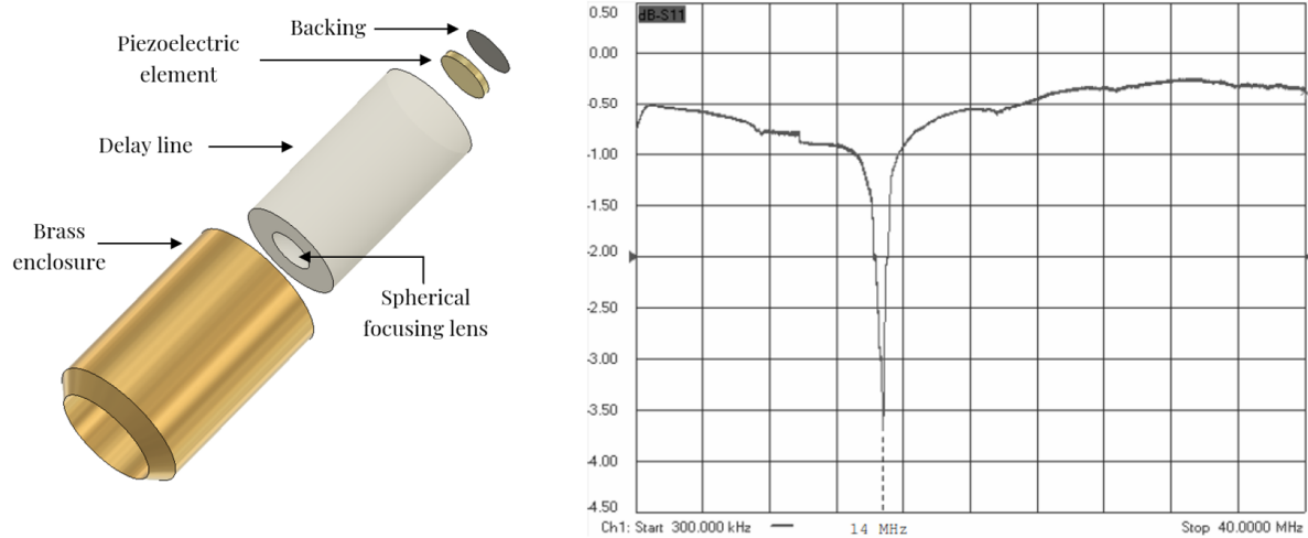
Fig. 5. Focused transducer design (left) and its Measured Reflection coefficient S11(dB) (amplitude of the reflected wave to the incident wave) as a function of frequency (right).
