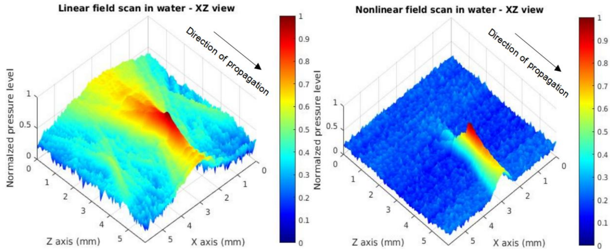
Fig. 8. Scanned focused ultrasonic fields in water: linear (14 MHz) field scan (left) and nonlinear (28 MHz) field scan (right).
