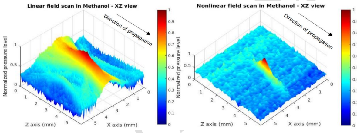
Fig. 10. Scanned ultrasonic focused fields in Methanol: linear (14 MHz) field (left) and nonlinear (28 MHz) field (right)
