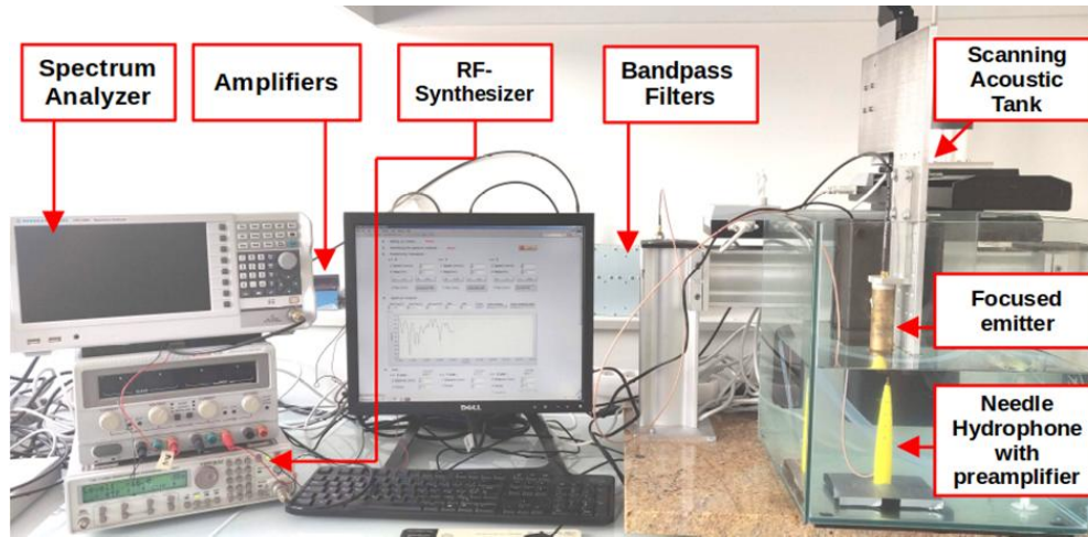
Fig. 7. Experimental measurement setup.
