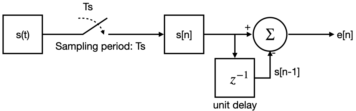
Fig. 4. Blockdiagram of proposed method. The signal "s(t)" is initially sampled with a period of "Ts". The error signal "e[n]" is obtained by subtracting the value of the sampled signal "s[n]" from its value in the previous period and recording it. In the next cycle, the same operations are continued by reducing the sampling period "Ts". The value of "e[n]" closest to zero corresponds to the period when the vibration period matches the sampling period.
