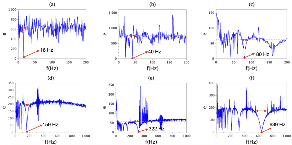
Fig. 8. Results of linear measurements with calibration device. According to the calibration device data, the true frequency values were measured as follows: a) 15.92 Hz, b) 40 Hz, c) 80 Hz, d) 159.2 Hz, e) 320 Hz, and f) 640 Hz.
