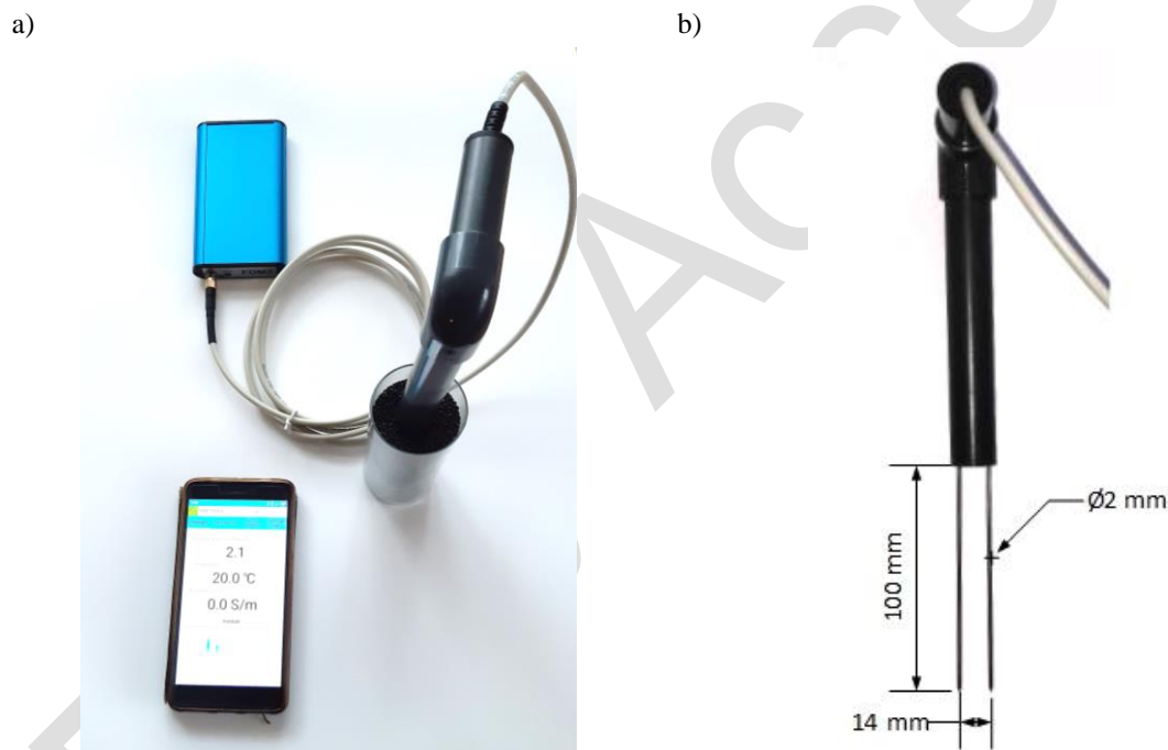
Fig. 2. a) Measurement setup, b) dimensions of the measuring probe.
