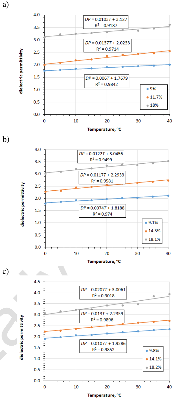
Fig. 5. Influence of temperature on dielectric permittivity for three levels of moisture content of three seed species: a) rapeseed, b) mustard, c) millet.
