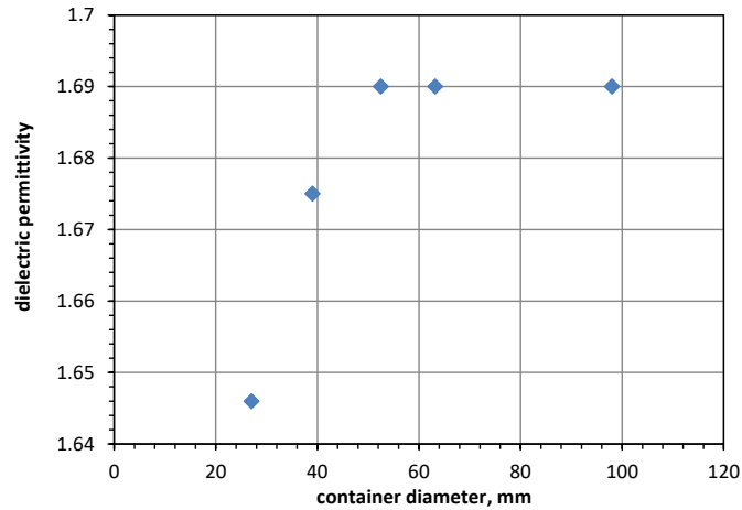
Fig. 3. Dependence of dielectric permittivity as a function of the diameter of the container for rapeseed with moisture of 5.2%.
