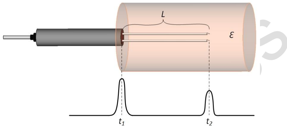
Fig.1. Principle of TDR measurement in a medium with apparent dielectric permittivity \epsilon . L is the length of the probe, t_1 and t_2 are the recorded time of the pulse reflected from the beginning and the end of the probe rods, respectively.
