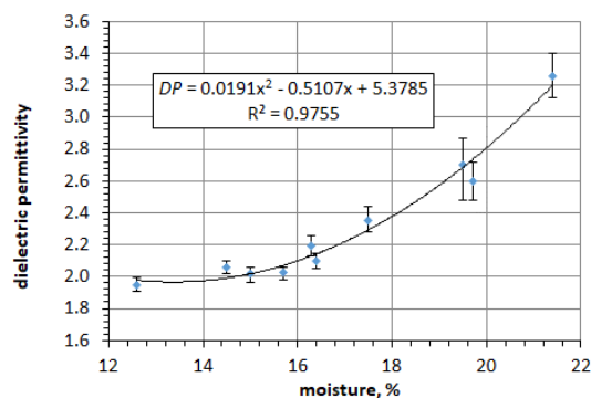
Fig. 4. Dependence of apparent dielectric permittivity (designated DP on the graphs) on seed moisture for: a) wheat, b) rapeseed, c) mustard, d) millet, e) common buckwheat, f) red clover, g) mixed alfalfa, h) tansy phacelia, i) maize, j) flax, k) persian clover, l) cannabis, m) soybean. Fitted models with R^2 were presented on the graphs.
