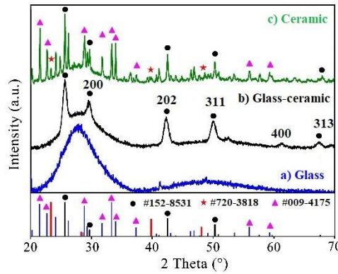
Fig. 1. X-ray diffraction patterns for Yb 3+ /Er 3+ co-doped (a) glass, (b) extruded glass-ceramic, and (c) glass heated at 560 °C for 30 minutes.
