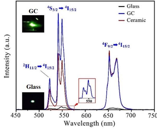
Fig. 4. Upconversion spectra of Yb 3+ /Er 3+ co-doped (a) glass, (b) extruded glass-ceramic, and (c) glass heated at 560 °C under 967 nm at room temperature.
