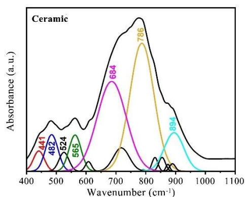
Fig. S3. FTIR spectra of Yb 3+ /Er 3+ co-doped germanium-tellurite matrix.
