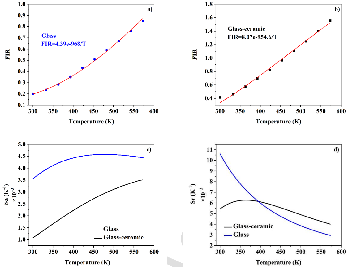
Fig. 8. (a), (b) Plot of FIR value versus absolute temperature and fitting curves, as well as (c), (d) relative temperature sensitivity S_a and S_r of glass and extruded glass-ceramic at various temperatures.
