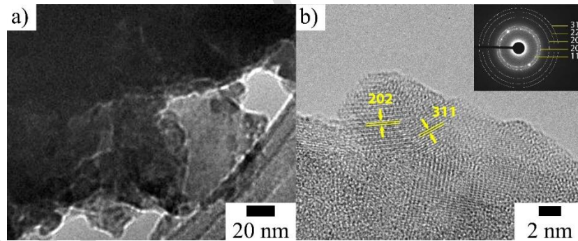
Fig. 2. TEM (a) and (b) HRTEM images for the extruded GC sample. The inset in (b) presents five diffraction rings originating from the diffraction of the lattice face with the Miller indices of (311) (222) (202) (200), and (111) – inset in 2b.
