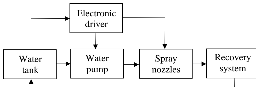
Fig. 3. Elements of the cooling system.
