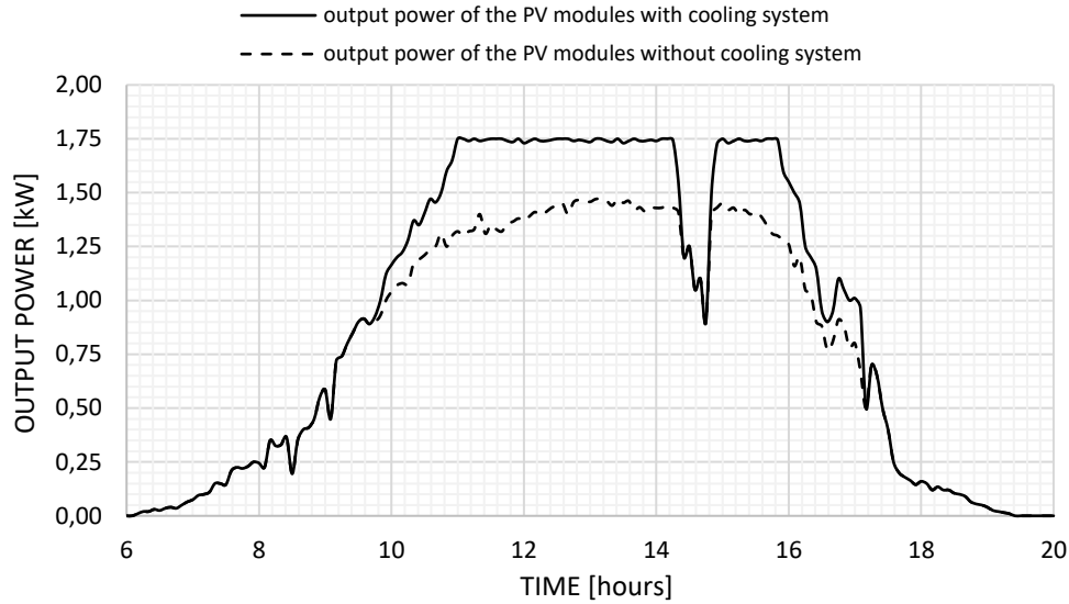
Fig. 6. Output power of the PV modules with and without the cooling system.
