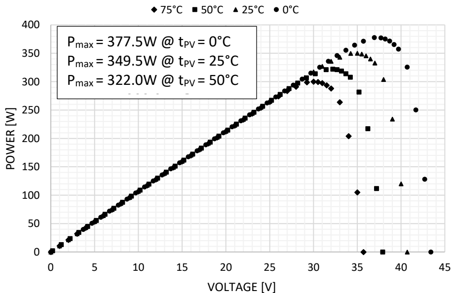
Fig. 1. The power-voltage characteristics of Q.PEAK DUO-G8 PV cell as a function of temperature for 0^\circ\text{C} , 25^\circ\text{C} , 50^\circ\text{C} and 75^\circ\text{C} .
