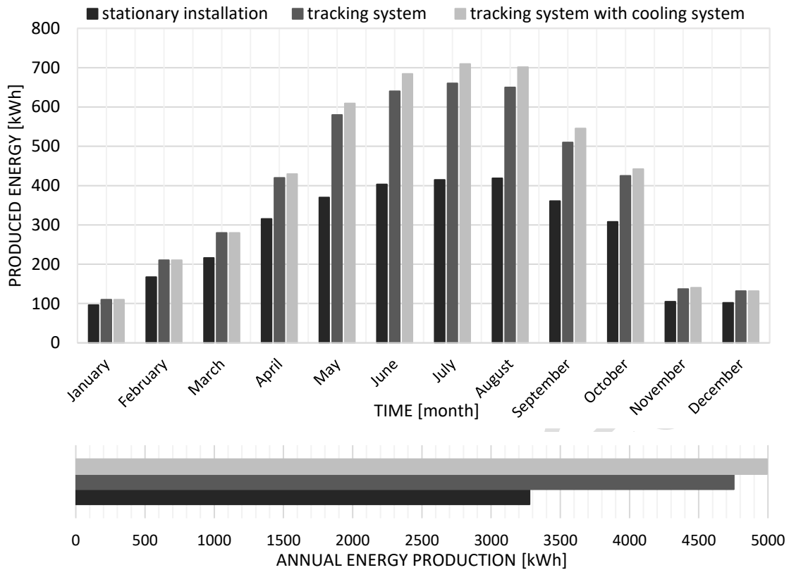
Fig. 9. Monthly energy production [kWh] by photovoltaic installation in stationary, tracking and tracking with cooling systems.
