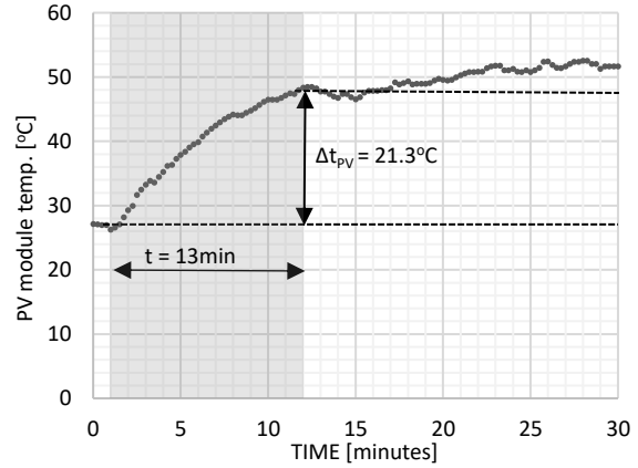
Fig. 5. The temperature change of the PV module after turning off the cooling system.
