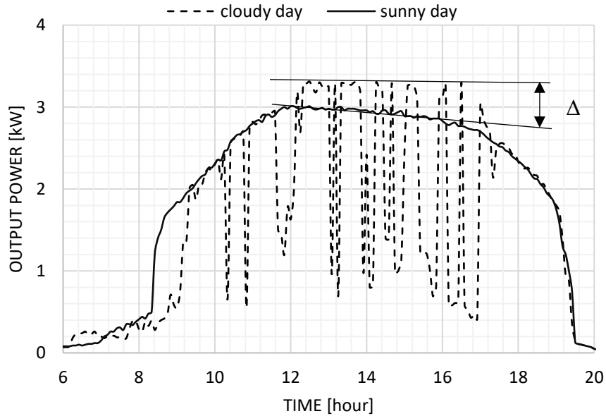
Fig. 2. Output power of the experimental setup on a temporary overcast and sunny day.
