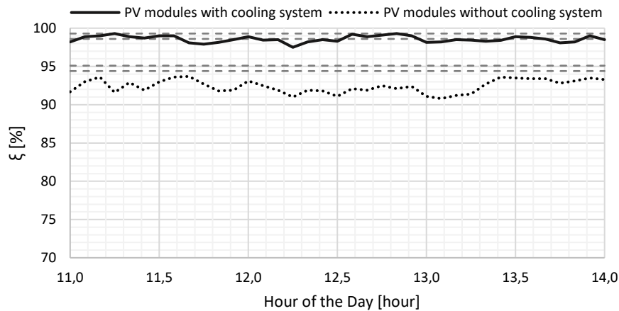
Fig 8. Value of the nominal efficiency of PV modules with the cooling system ( t_{PV} = 27-29\text{ }^{\circ}\text{C} ) and without the cooling system ( t_{PV} = 33-35\text{ }^{\circ}\text{C} ).
