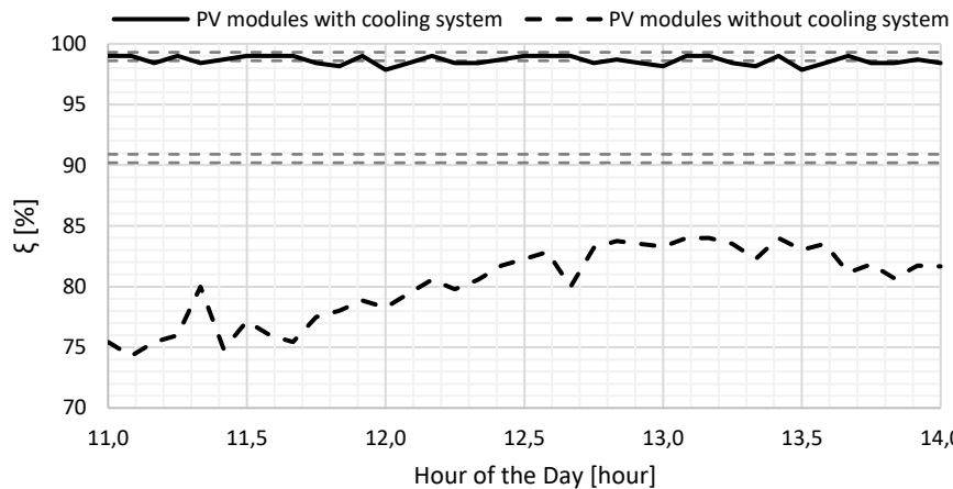
Fig 7. Value of the nominal efficiency of PV modules with the cooling system ( t_{PV} = 27-29 °C) and without the cooling system ( t_{PV} = 51-53 °C).
