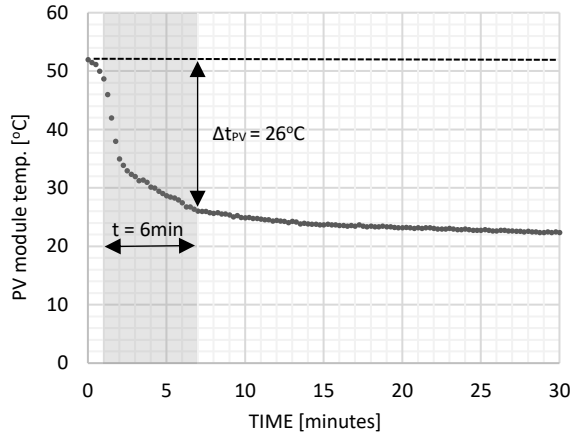
Fig. 4. Temperature change of the PV module after turning on the cooling system.
