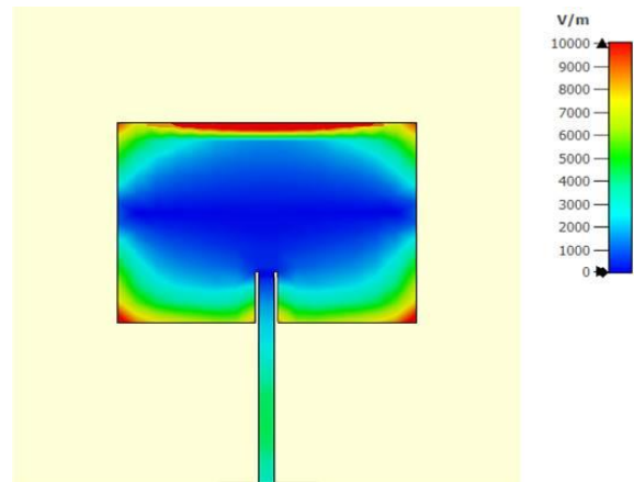
Fig. 3. Electric field distribution on the patch.
