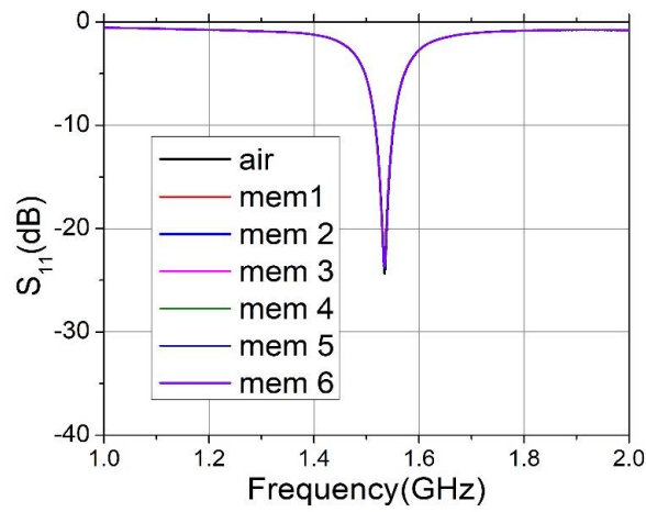
Fig. 10. S_{11} parameters for an empty cavity followed by each measurement.
