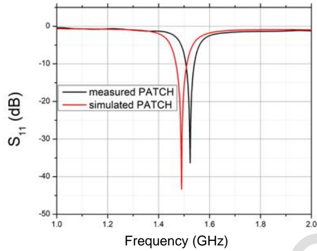
Fig. 6. Measured result vs. simulated result for the microstrip patch antenna.
