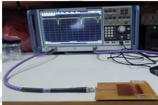
Fig. 5. Experimental setup of the microwave sensor.
