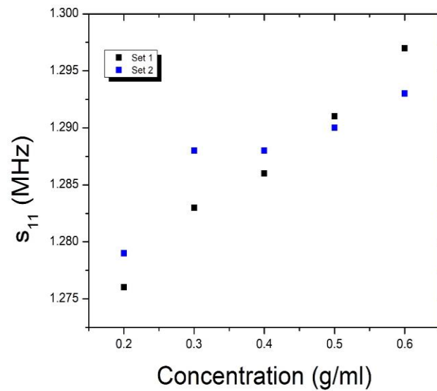
Fig. 12. Stability graph of frequency for the repeated experiment.
