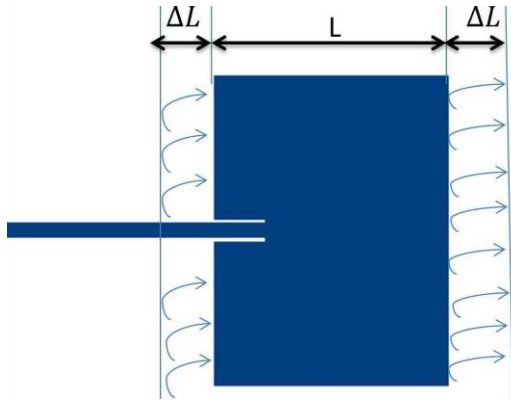
Fig. 2. Fringing fields along the patch edge length.
