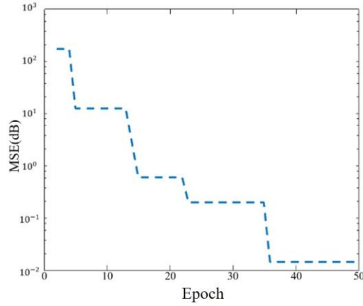
Fig. 5. Convergence curve of GRNN.
