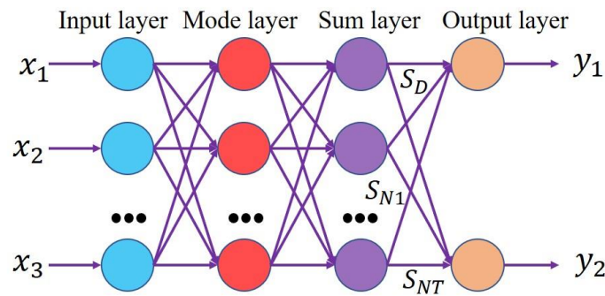
Fig. 4. GRNN structure.
