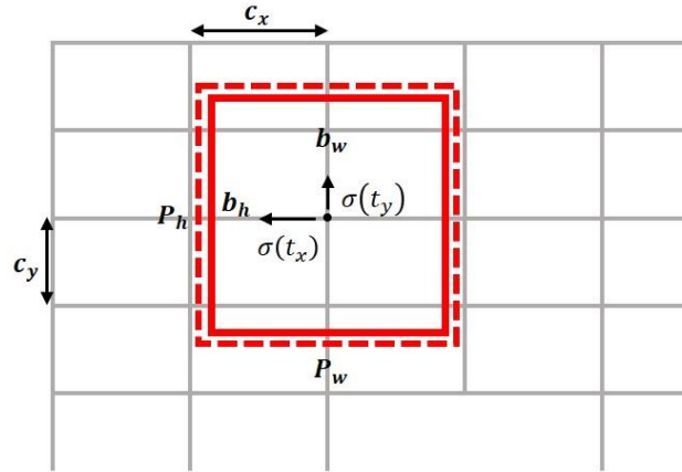
Fig. 11. Bounding box coordinate diagram.
