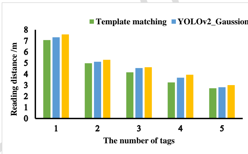
Fig. 14. The maximum reading distance corresponding the tag group.
