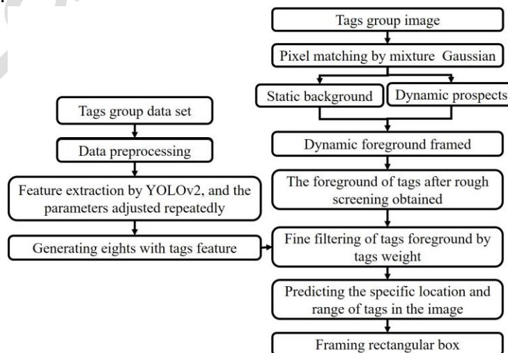
Fig. 8. Flow chart of tags group recognition algorithm YOLOv2 improved by Gaussian.
