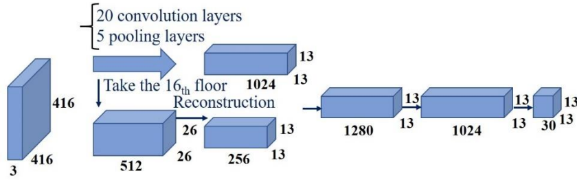
Fig. 10. YOLOv2 network structure.
