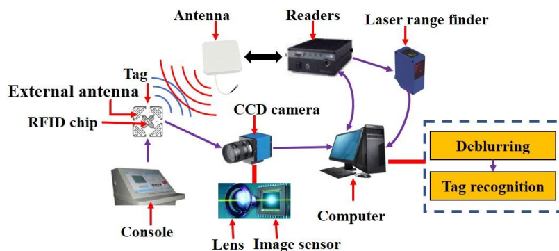
Fig. 1. Structure diagram of RFID tag group recognition measurement system.
