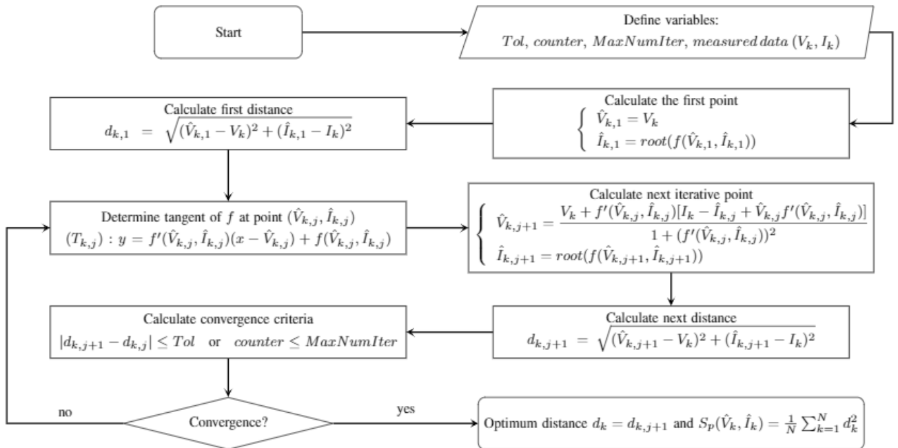
Fig. 3. Flowchart of optimum distance calculation through the TLS approach.
