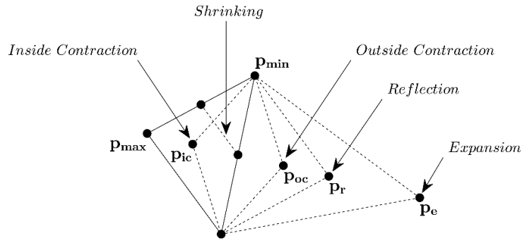
Fig. 4. Illustration of Nelder-Mead algorithm.
