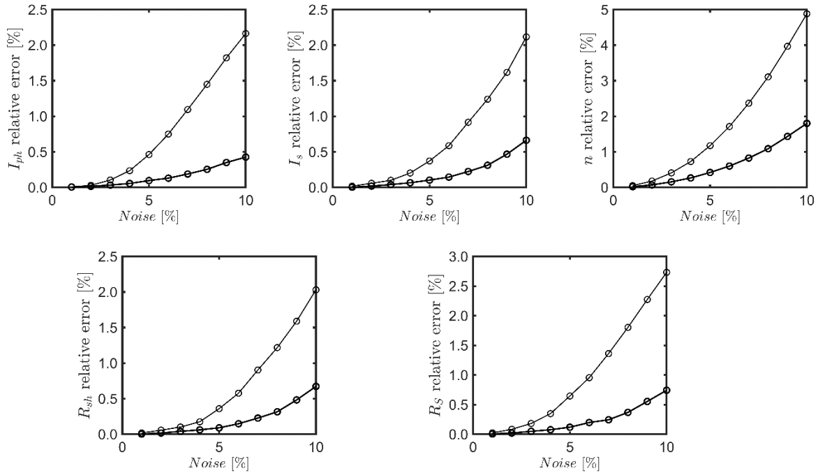
Fig. 7. Relative error values of the estimated photovoltaic parameters. The thin line corresponds to the OLS results while the thick line corresponds to the TLS results.
