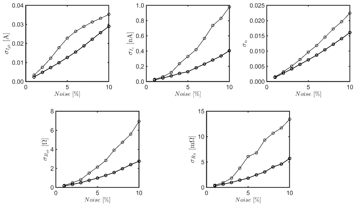
Fig. 6. Standard deviation of the estimated photovoltaic parameters. The thin line corresponds to the OLS results while the thick line corresponds to the TLS results.
