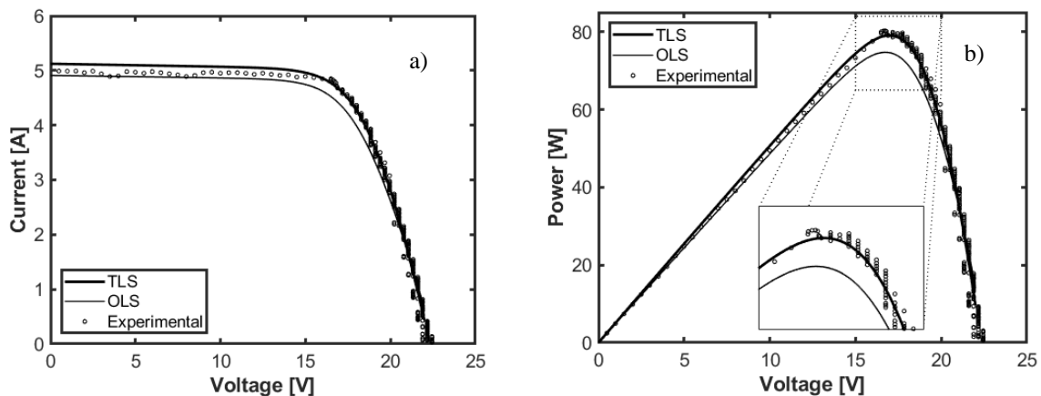
Fig. 9. a) Experimental I-V characteristic along with the characteristics obtained with the TLS and OLS single-diode model estimated parameters. b) Experimental P-V characteristic along with the characteristics obtained with the TLS and OLS single-diode model estimated parameters.
