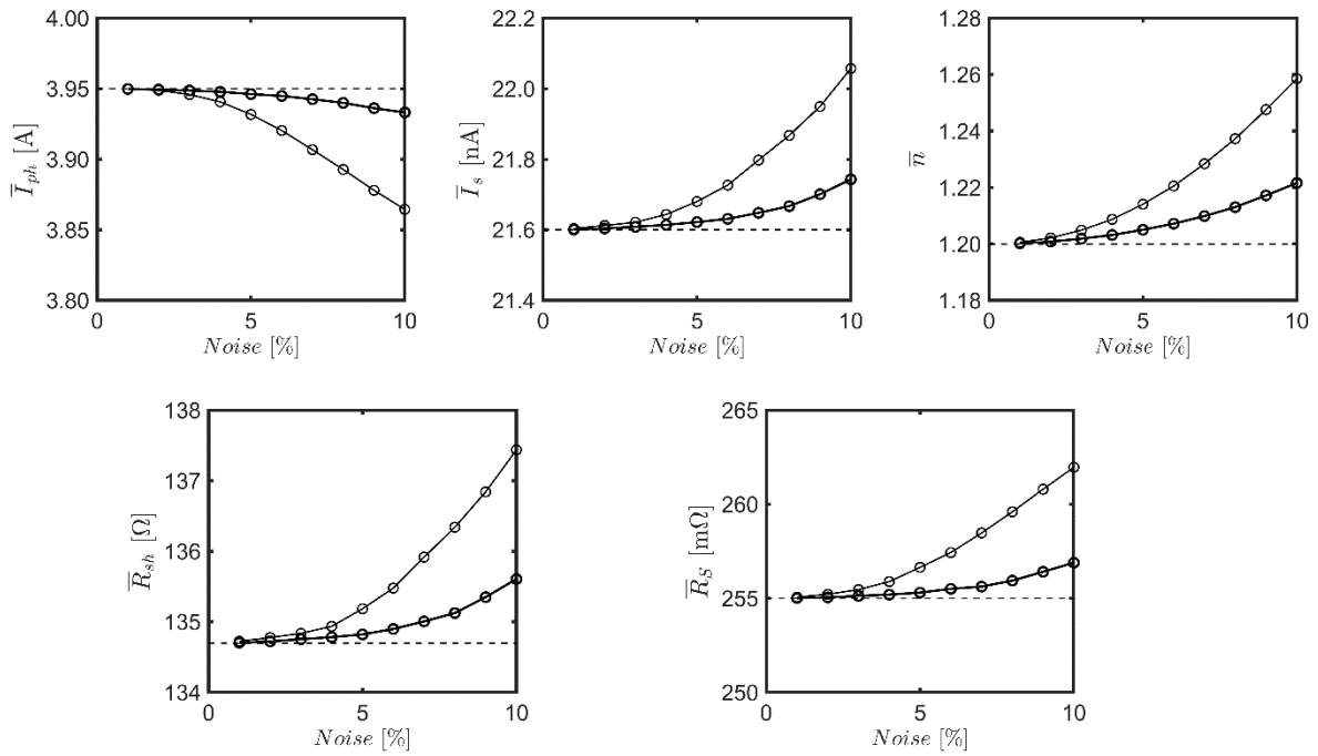
Fig. 5. Average values of the estimated photovoltaic parameters. The thin line corresponds to the OLS results while the thick line corresponds to the TLS results. The dashed line represents the reference value of each parameter.
