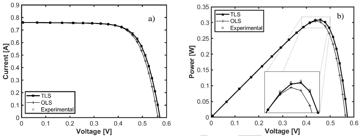
Fig. 8. A) Experimental I-V characteristic along with the characteristics obtained with the TLS and OLS for silicon cell from R.T.C France. B) Experimental P-V characteristic along with the characteristics obtained with the TLS and OLS silicon cell from R.T.C France.
